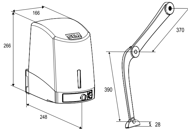
DIMENSIONS (mm)
