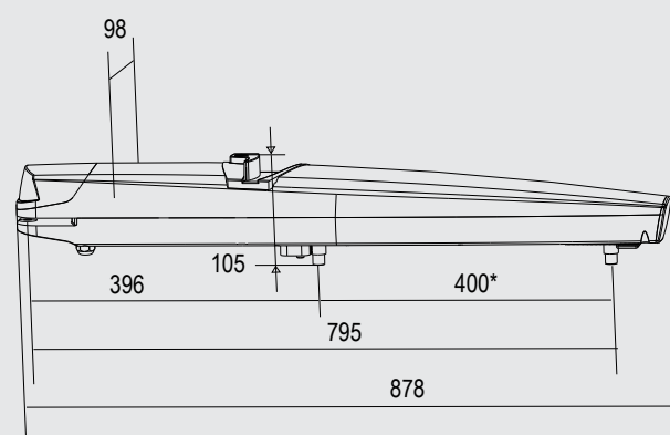
DIMENSIONS (mm)
